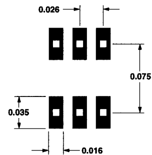
Figure 16. PCB Pad Layout (dimensions in inches).
