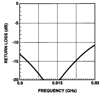
Figure 12. Input Return Loss.
