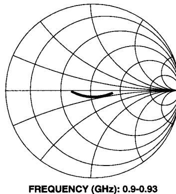
Figure 11. Input Impedance.
